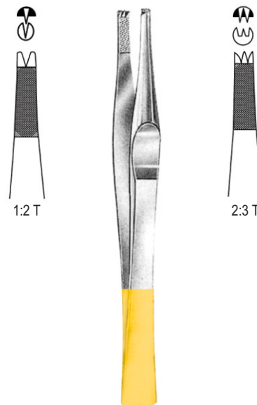
LANES 11.5166.12 12.5cm 11.5168.12 11.5166.15 15.5cm 11.5168.15 11.5166.18 18.0cm 11.5168.18 11.5166.20 20.0cm 11.5168.20
