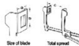
Scheme of dimensions
