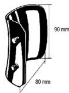
S/S Alu 36.0491.90 36.7491.90 80x90mm
